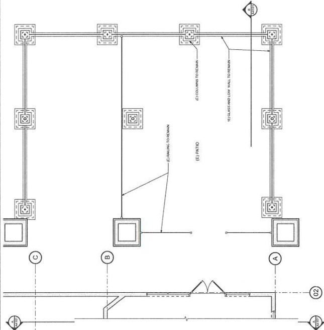
FIRST FLOOR DEMOLITION PLAN (PATIO)
