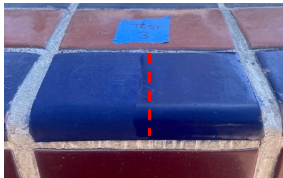
Area of west interior vertical surface after treatment with IBIX® system using sodium bicarbonate media followed by an additional pass with Stone Pro® Stone & Glass Scrub undiluted.
