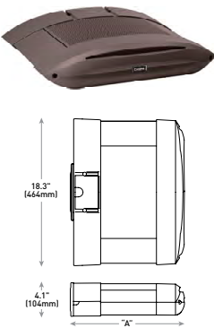
EDGE: WALL MOUNTED LIGHT FIXTURE MANUFACTURER: CREE LIGHTING COLOR: BRONZE
