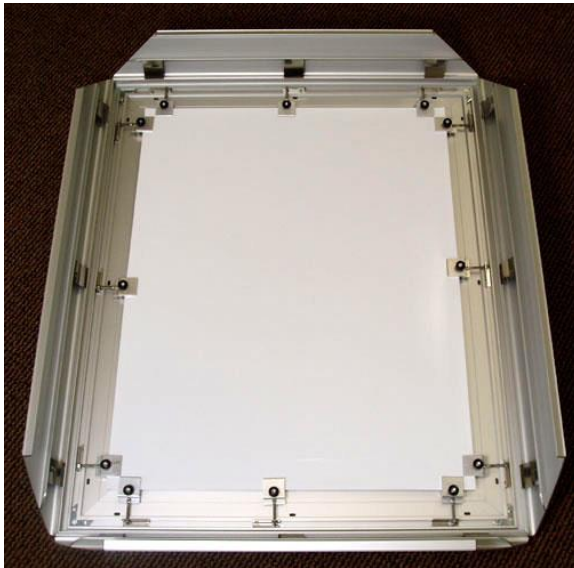
Above: Open frame to reveal clamps pulling banner tight.
